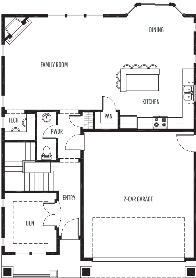
MAIN LEVEL
