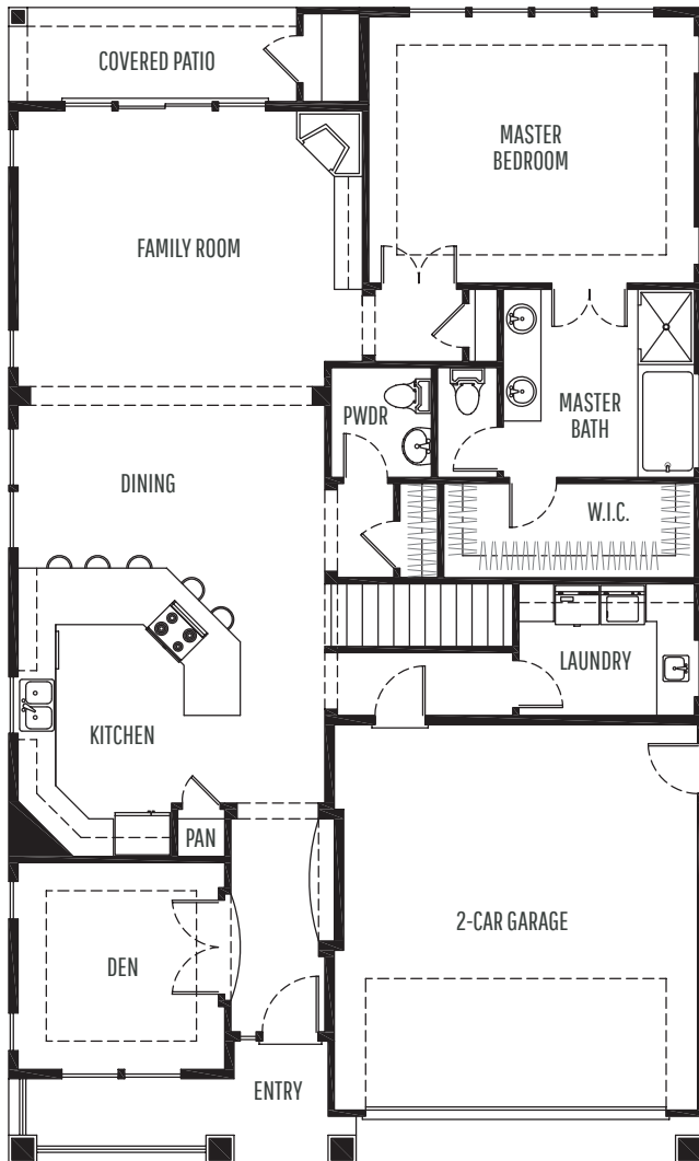
MAIN LEVEL
