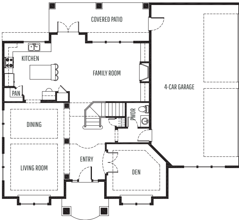
MAIN LEVEL
