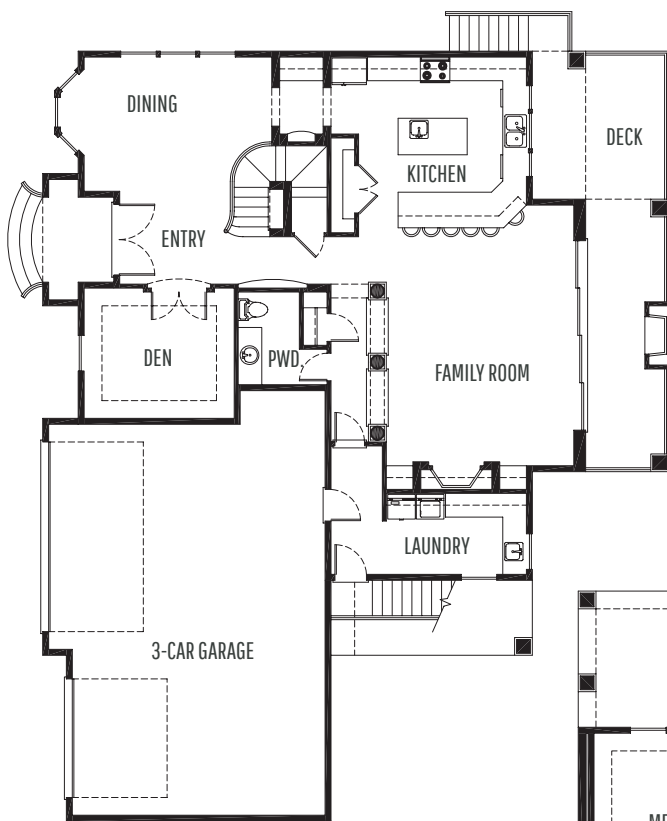
MAIN LEVEL
