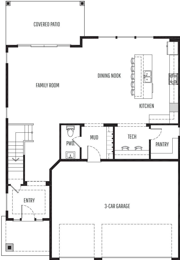
MAIN LEVEL
