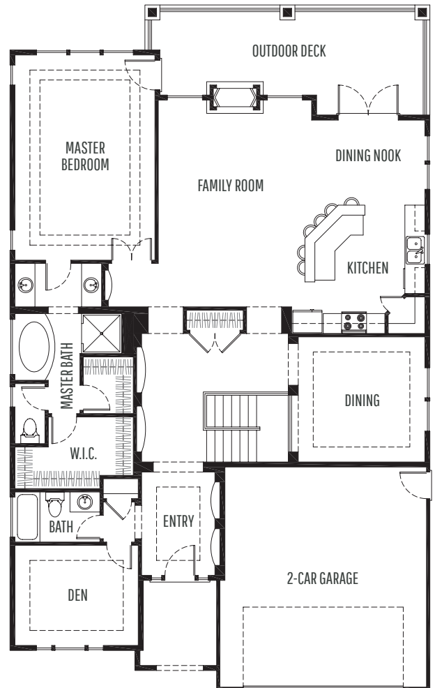
MAIN LEVEL
