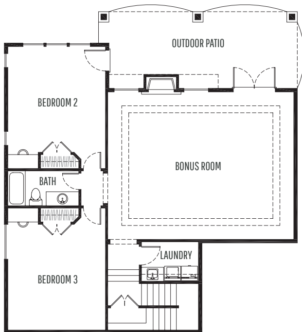
LOWER LEVEL
