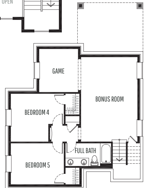
LOWER LEVEL
