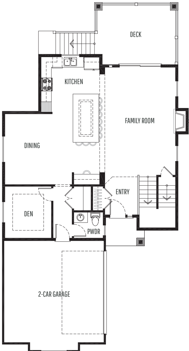
MAIN LEVEL
