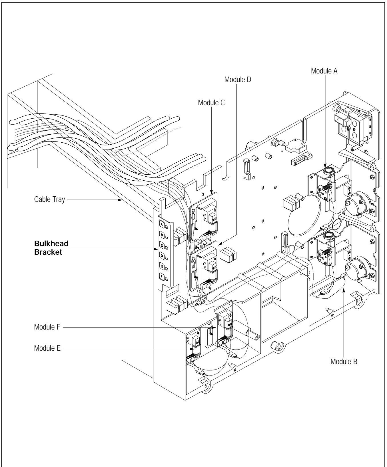
Figure 16. Modules C and D Mounted on HP 5890 Series II GC Built after January, 1992 (Sheet 2 of 2).
