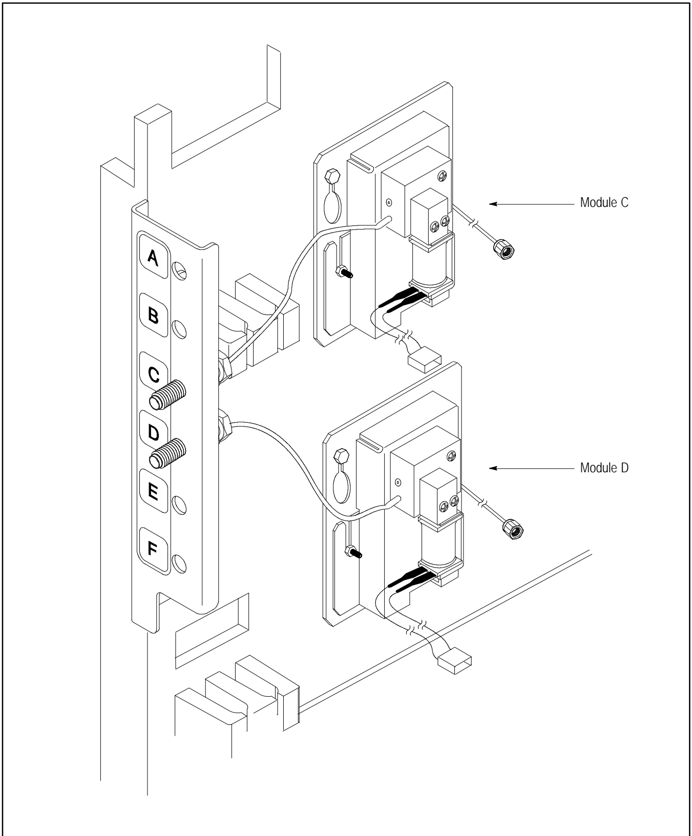
Figure 15. Modules C and D Mounted on HP 5890 Series II GC Built after January, 1992 (Sheet 1 of 2).
