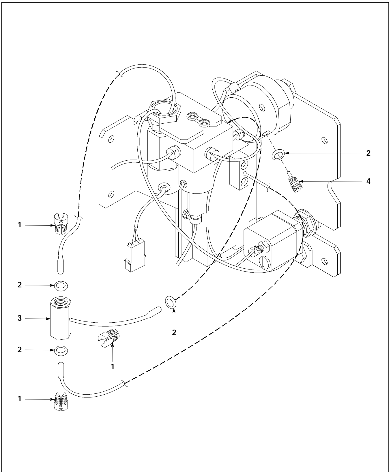
Figure 3. Back Pressure Controlled Split/Splitless Capillary Inlet (Sheet 2 of 2).
