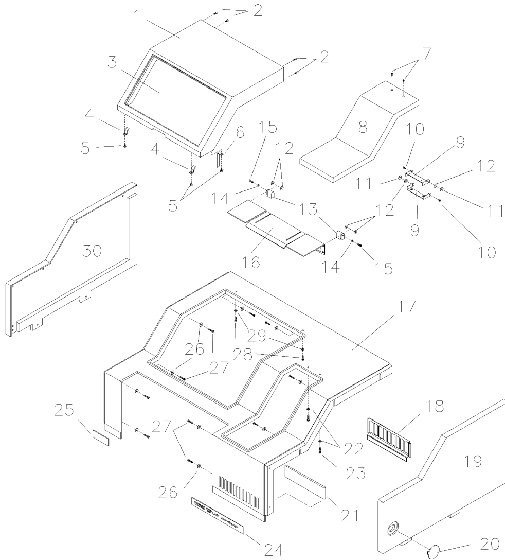
Figure 4-1. Top Cover
