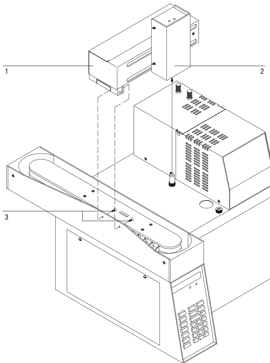
Figure 2-1. Removing the Loader Unit
