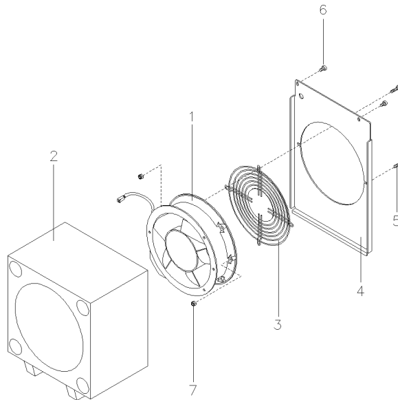
Figure 4-4. DC Fan Parts
