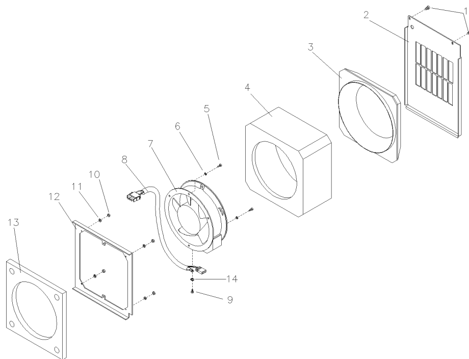
Figure 4-5. AC Fan Parts
