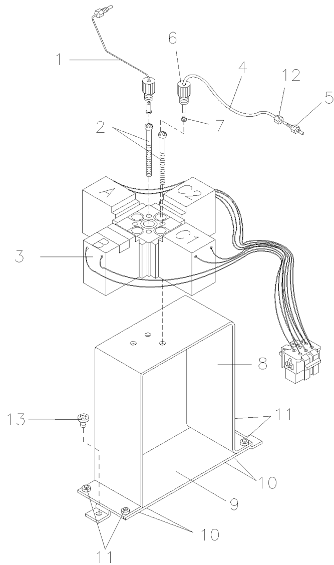
Figure 23-1. MGV Parts
