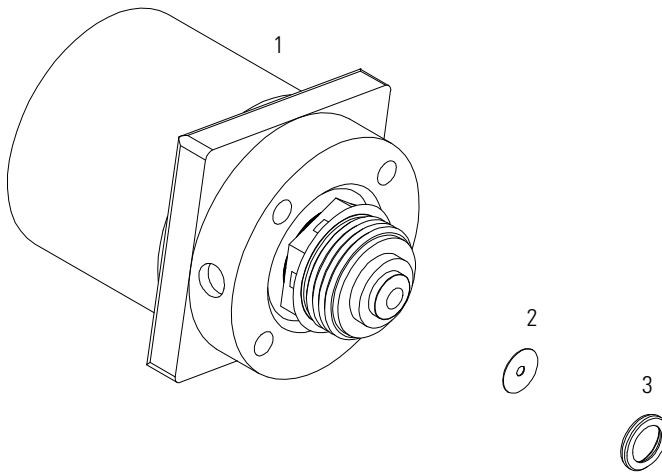
Active Inlet Valve Assembly
