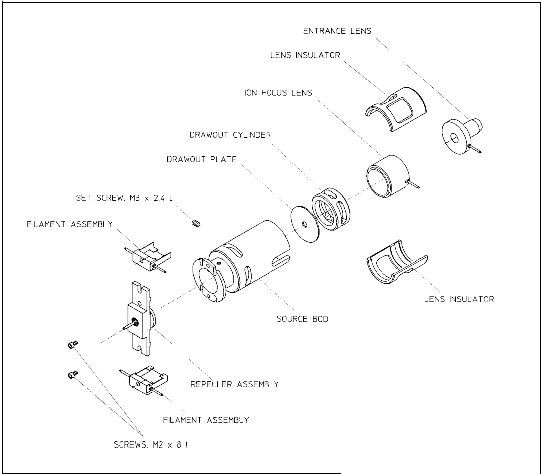
Figure 7-2. Ion source - exploded view
