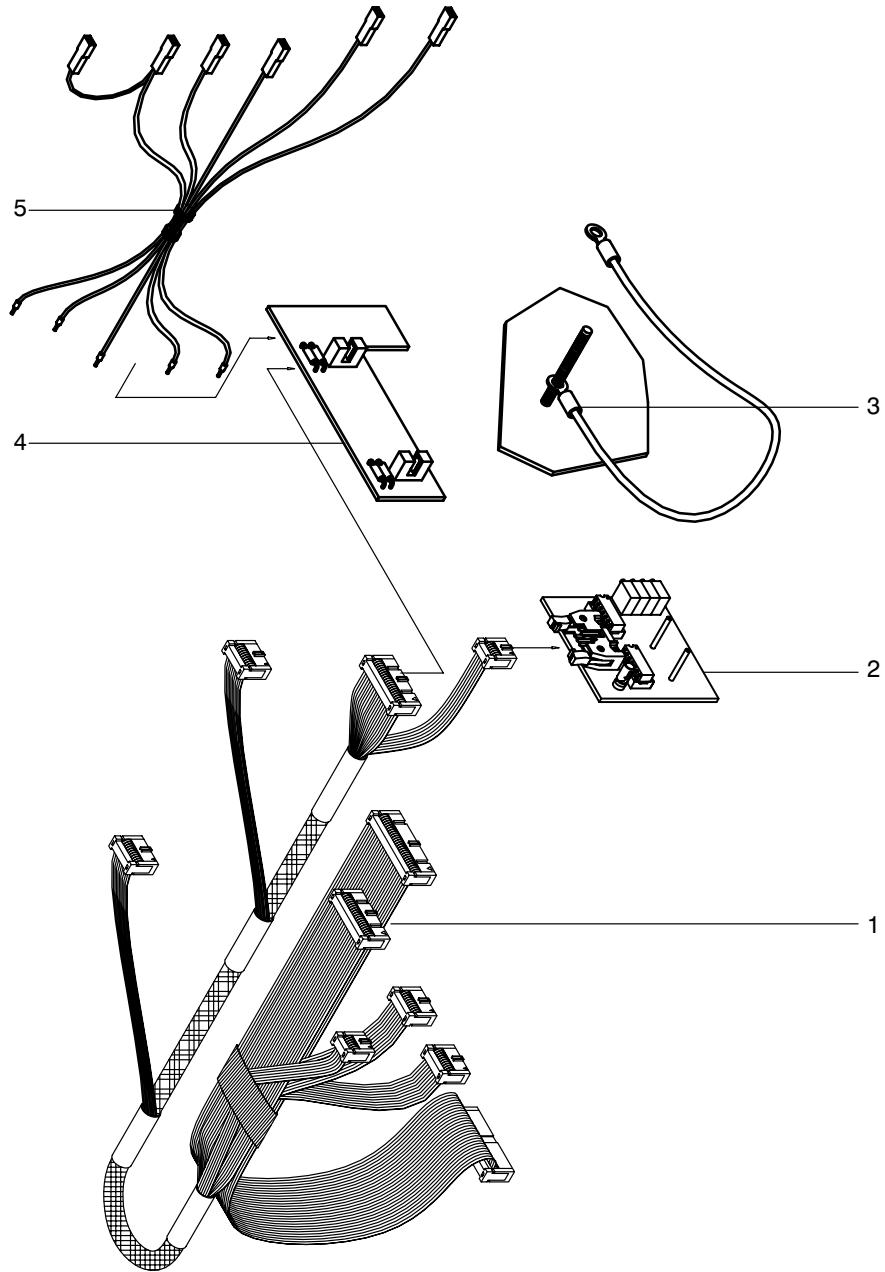
Figure 8-2. Sampler Unit Group
