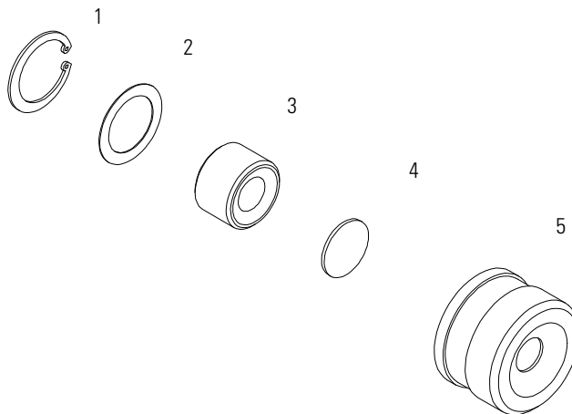
Coupling Lens Assembly Parts
