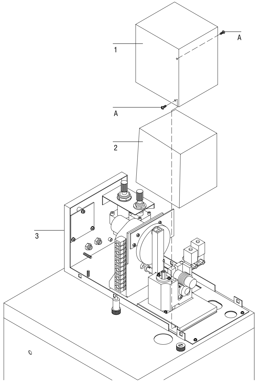
Figure 5-3. Insulation
