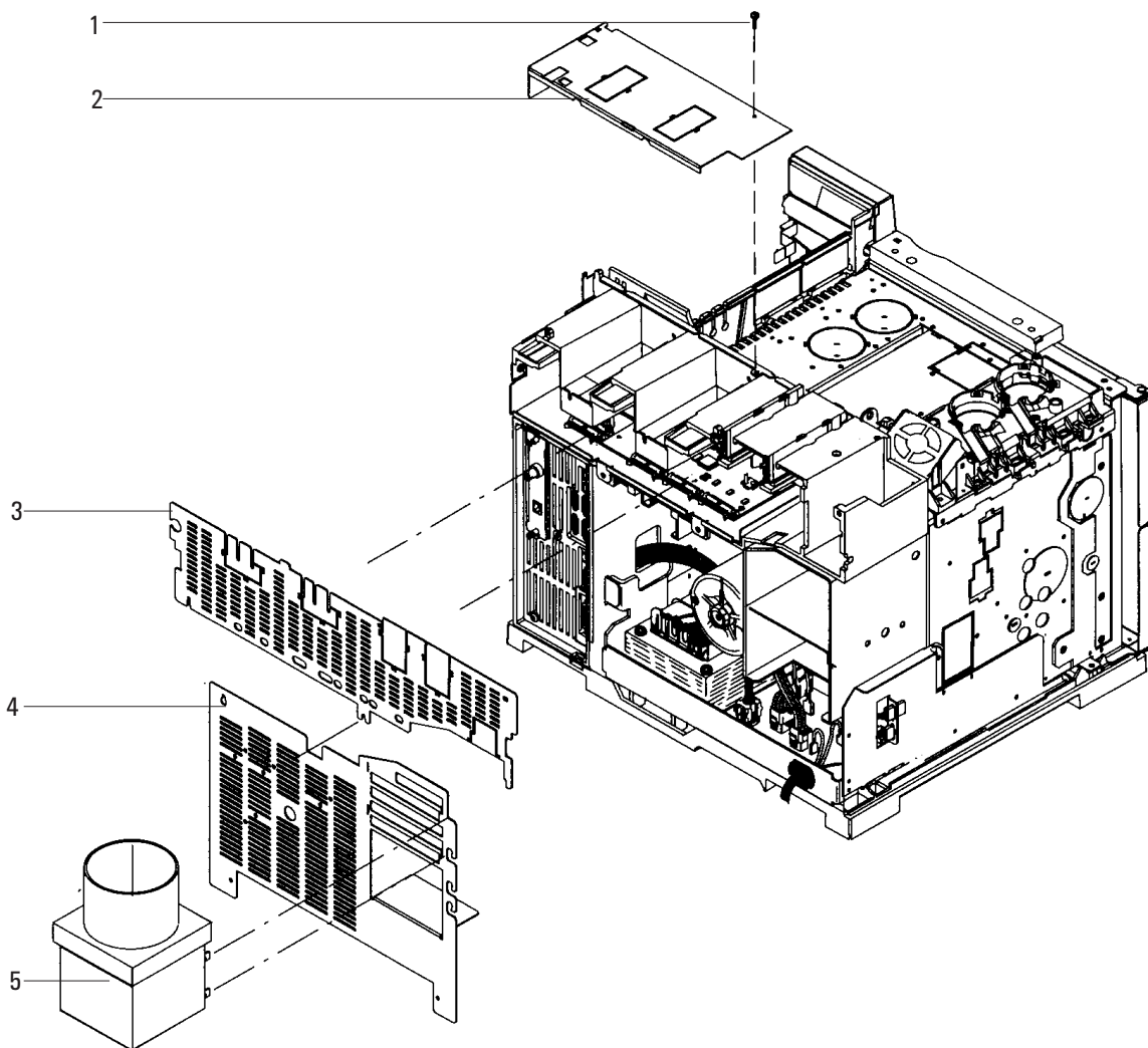
Figure 1330-1 Exploded diagram of the metal exterior components.
