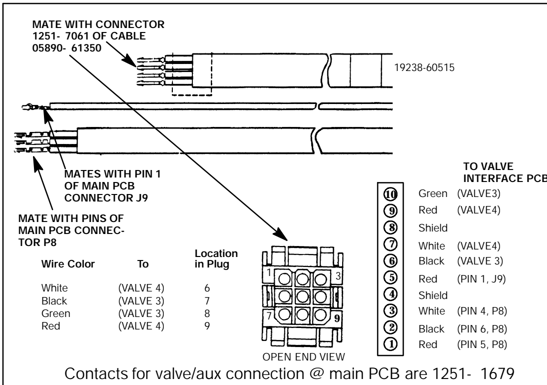
Figure 10. Valve Control Cables (Sheet 1 of 2).
