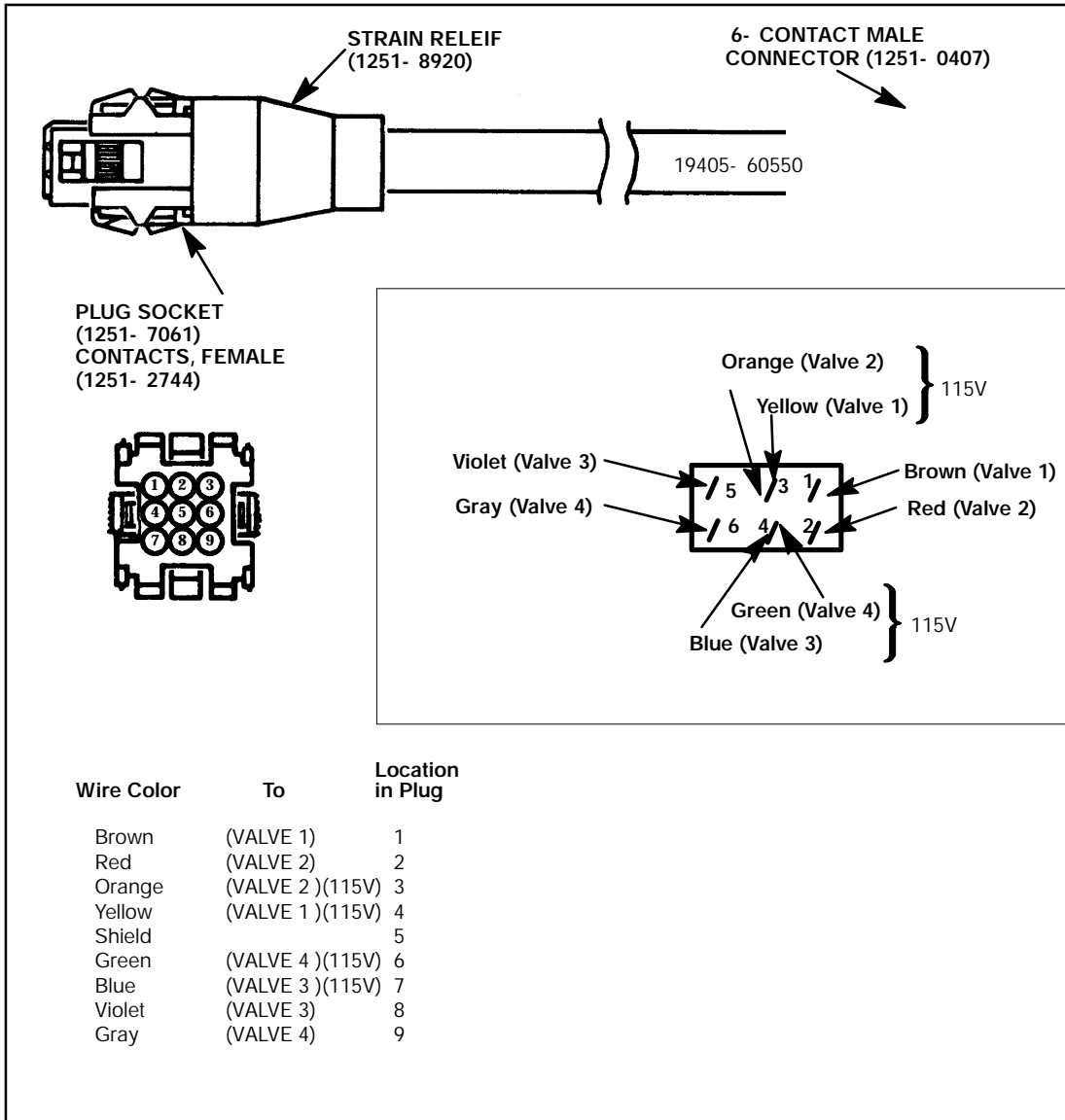
Figure 10. Valve Control Cables (Sheet 2 of 2).
