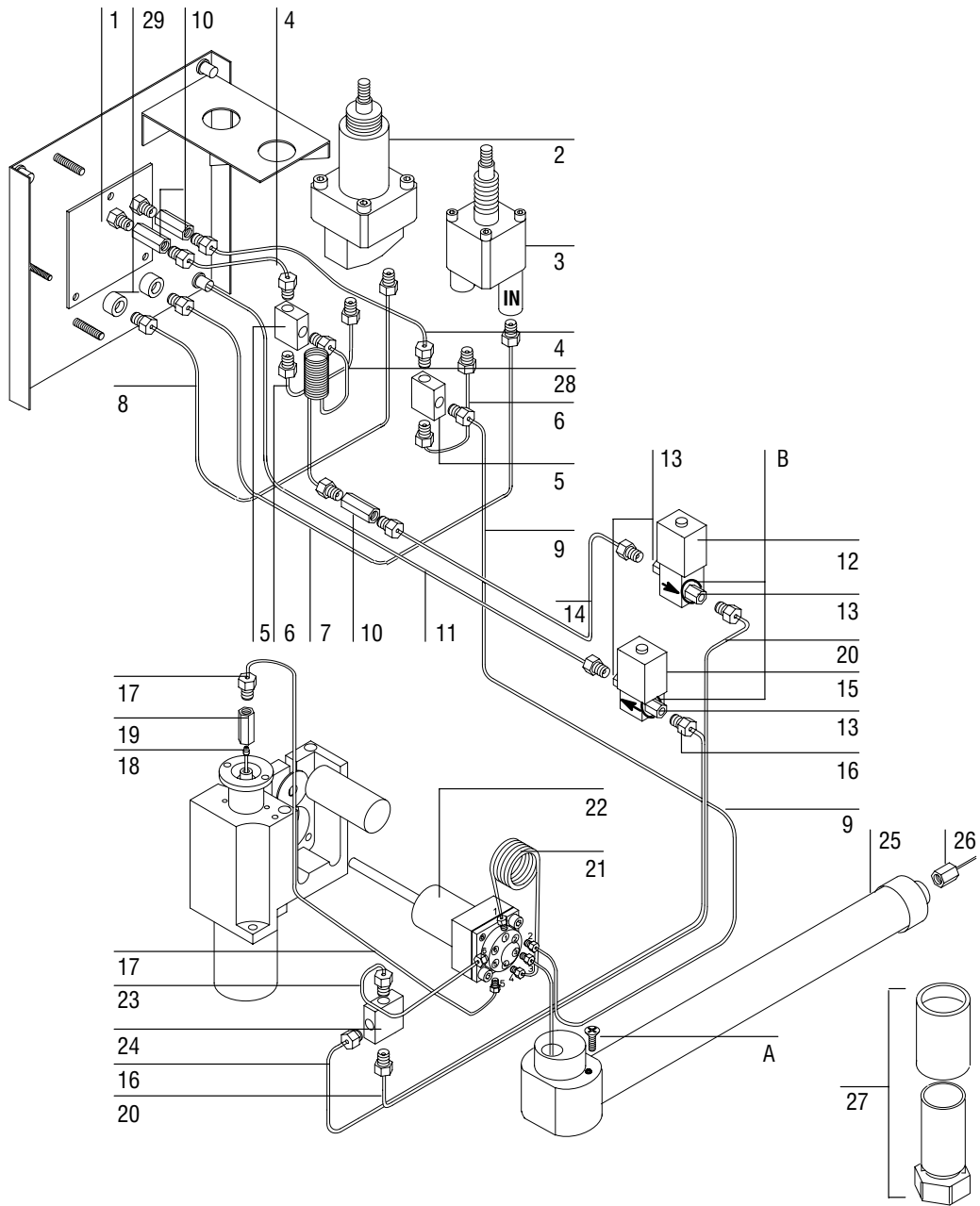
Figure 5-4. Plumbing Diagram (Stand Alone version)
