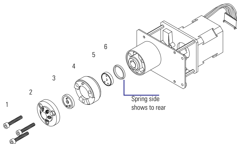
Column Switching Valve Parts
