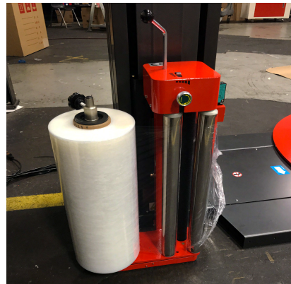
Film Carriage Assembly
