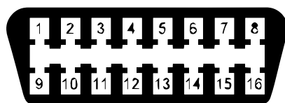
Figure 2 - Vehicle OBDII Connector
