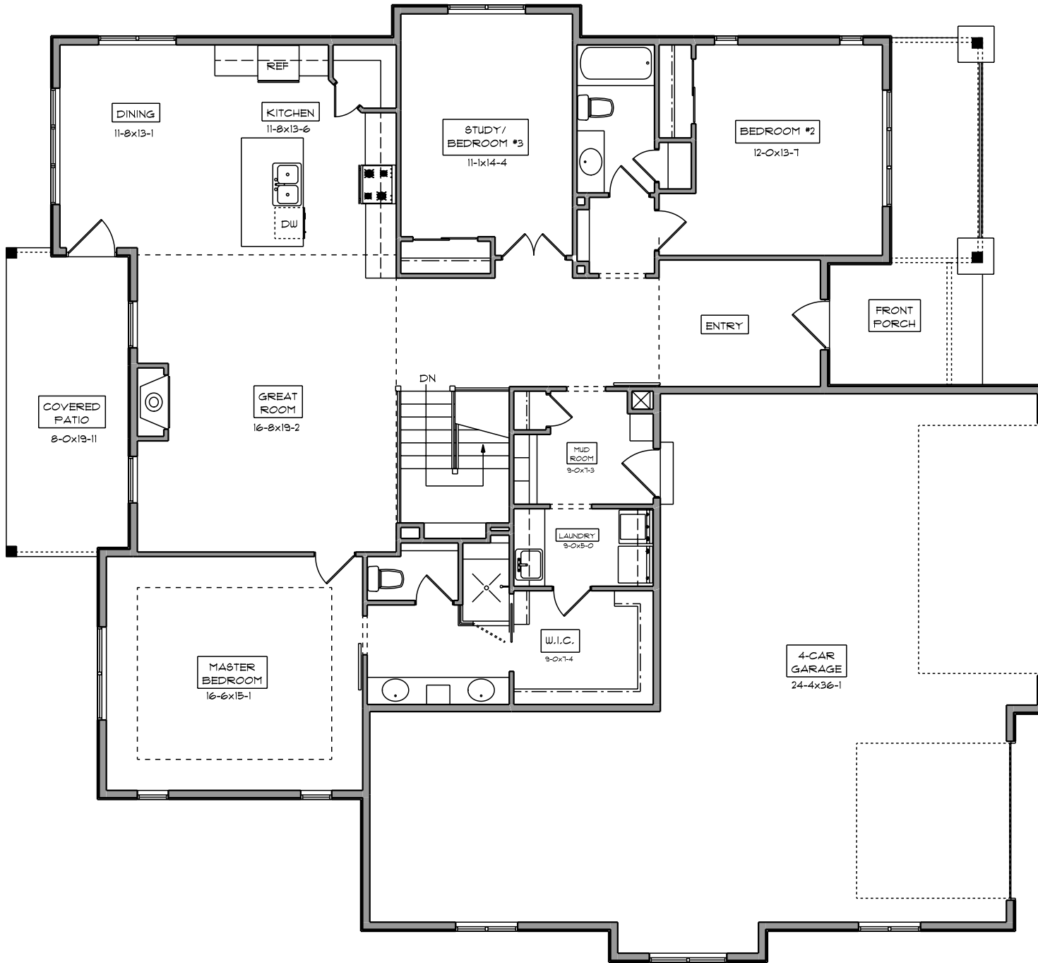
MAIN FLOOR PLAN 2,004 FinSqFt
