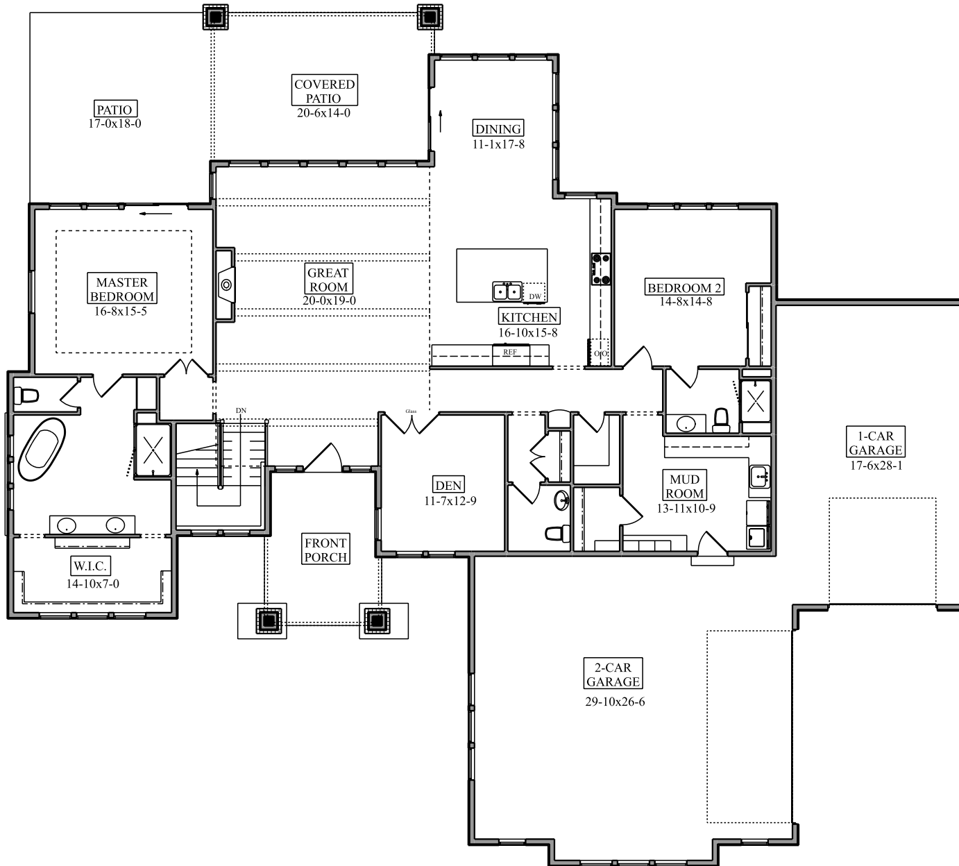
MAIN FLOOR PLAN 2,593 FinSqFt
