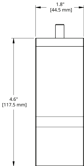
FRONT VIEW
